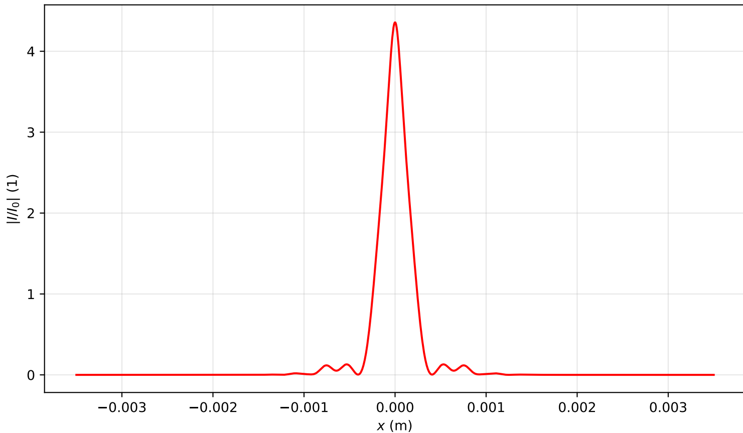
Intensity profile I(x, y = 0, z = 0.716)/I_0 , P_{in}=8.0P_{cr} , artificial time
